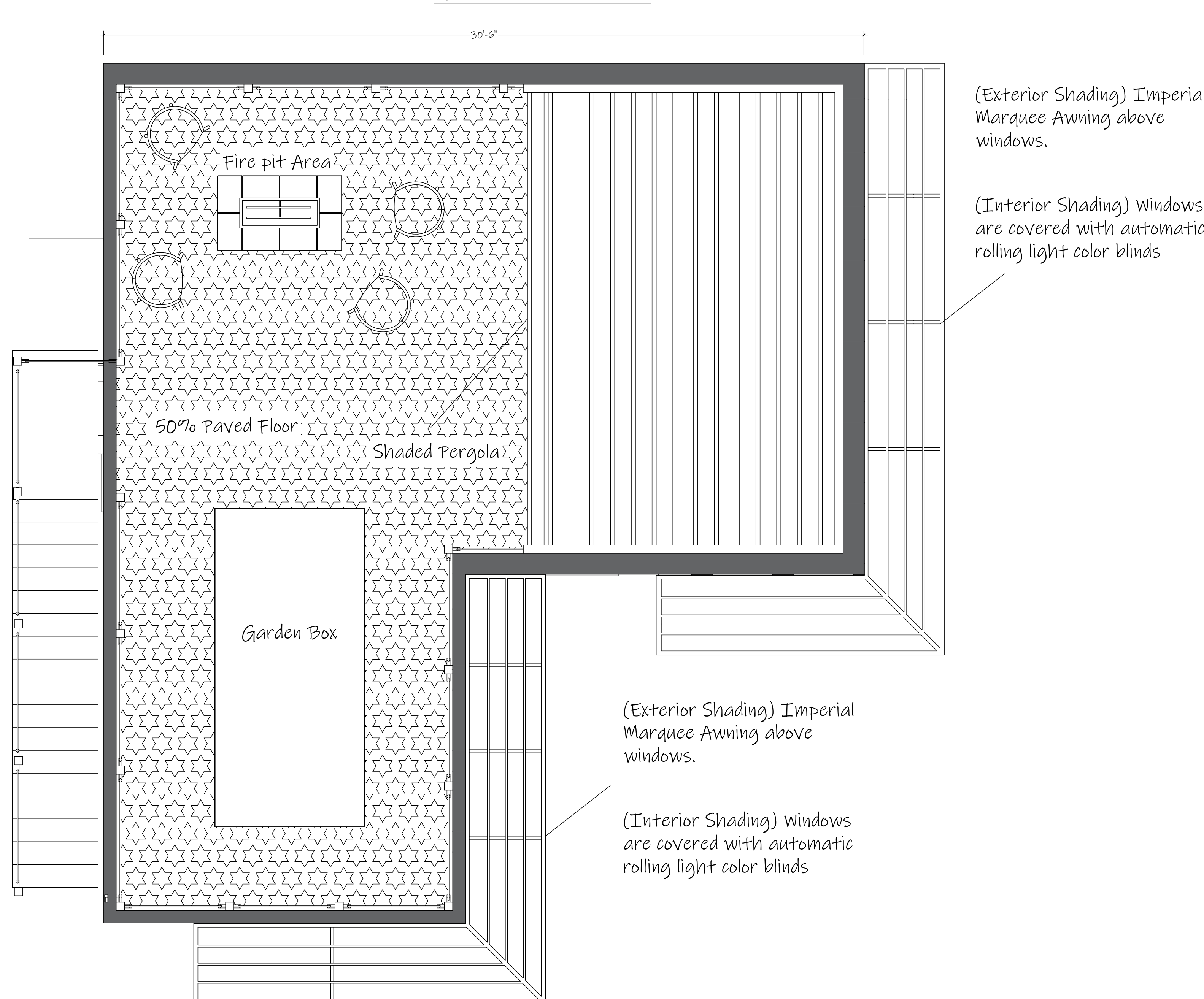
GREEN ROOF TOP PLAN
