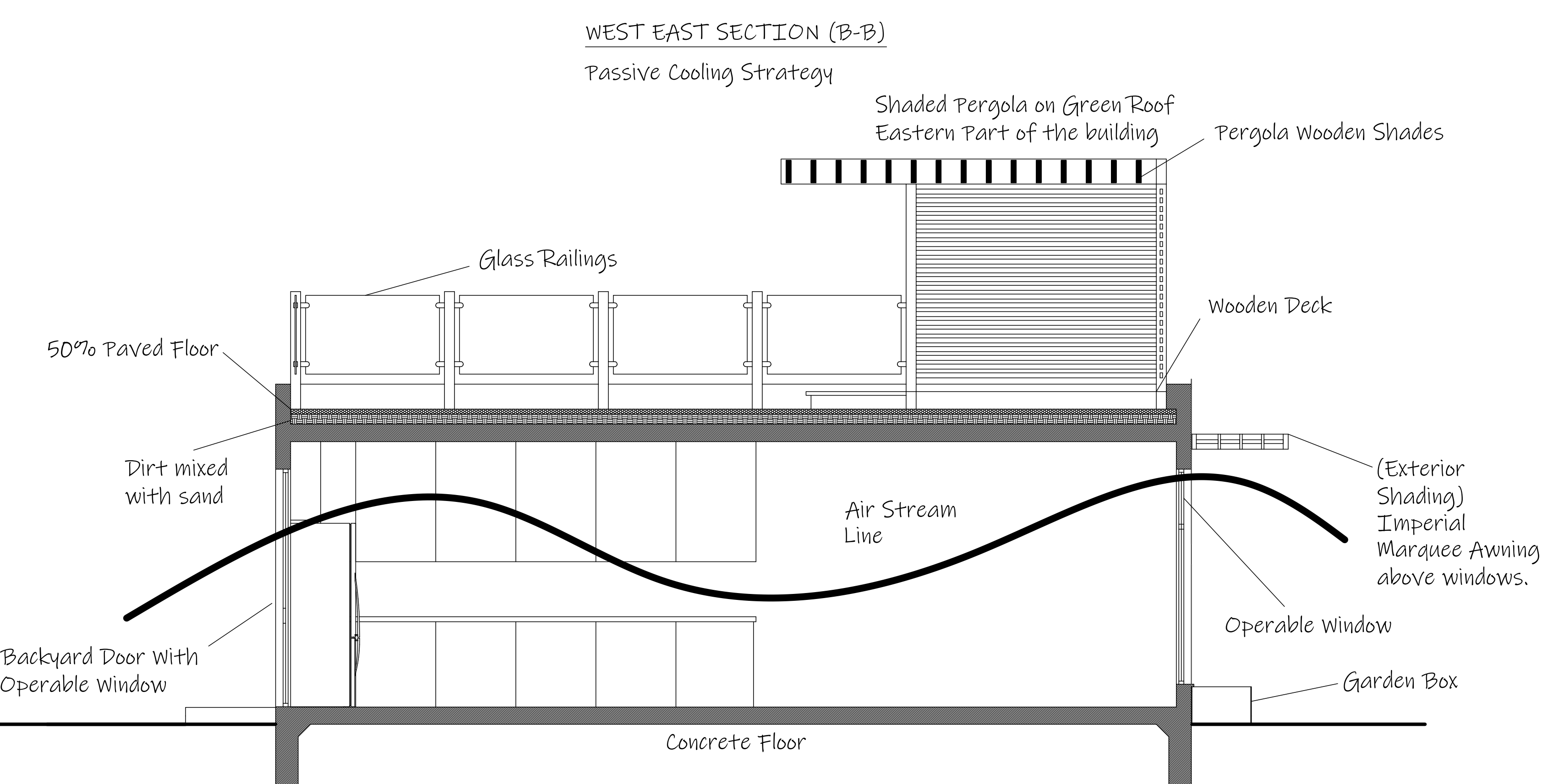
WEST EAST SECTION (B-B)
