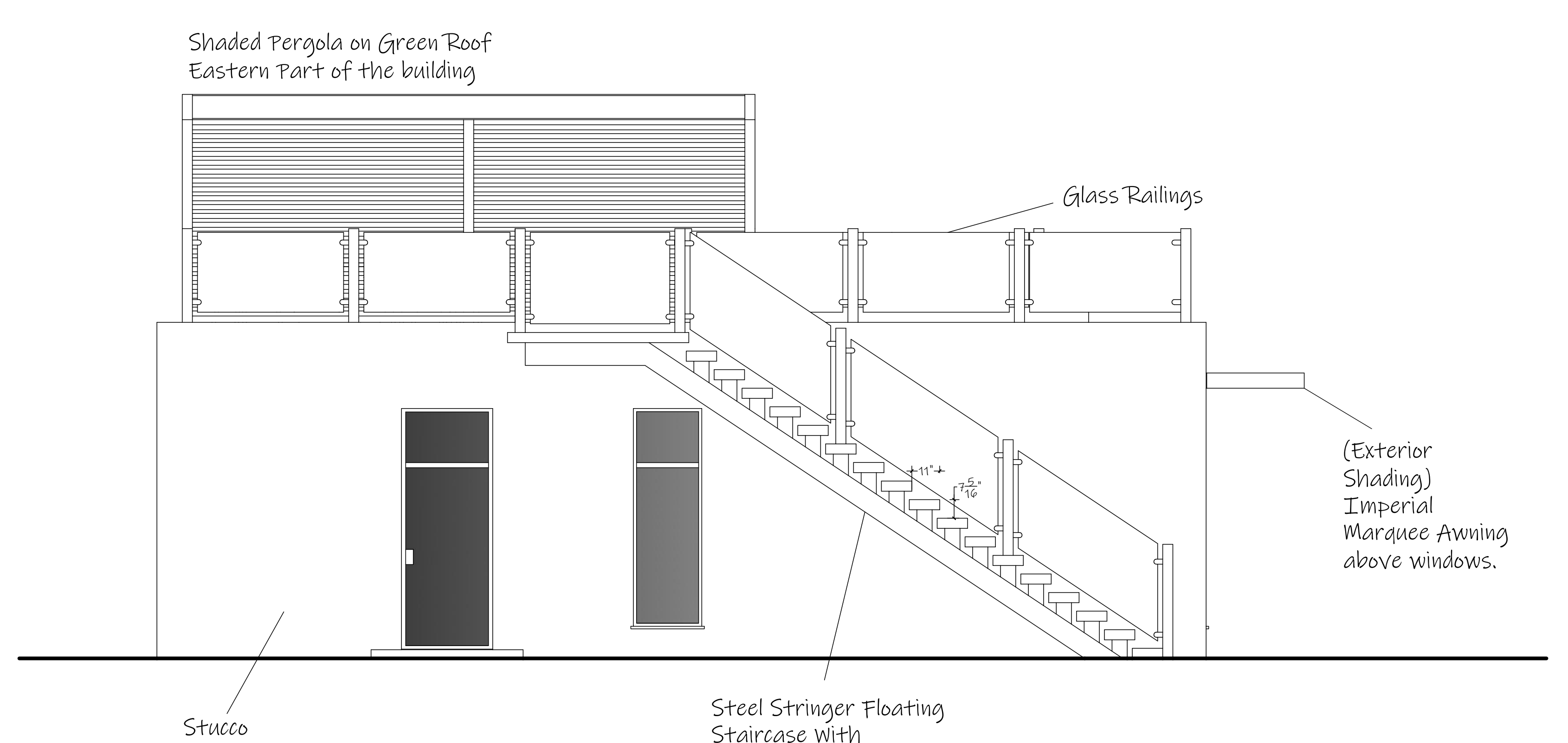
WEST ELEVATION
