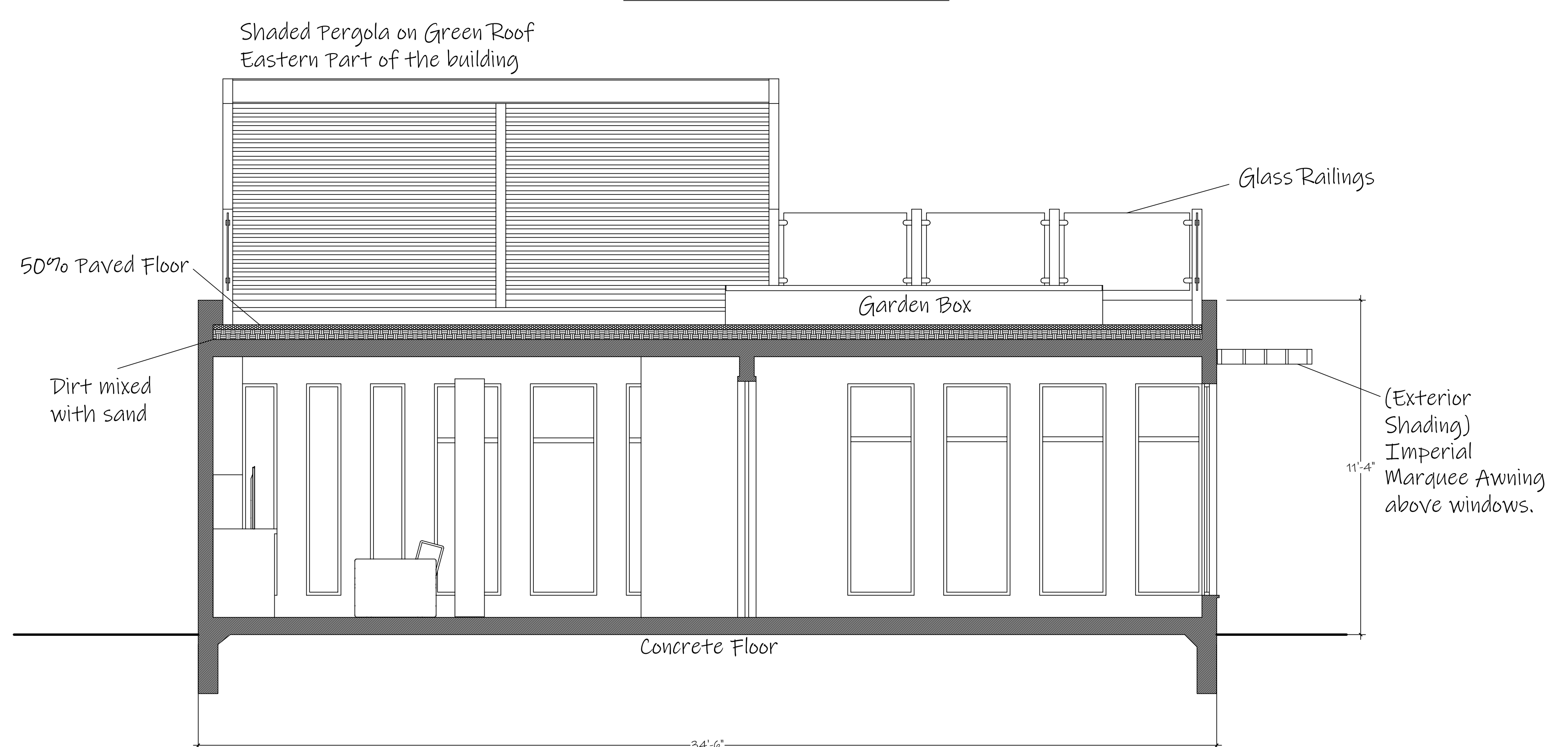
SOUTH NORTH SECTION (A-A)
